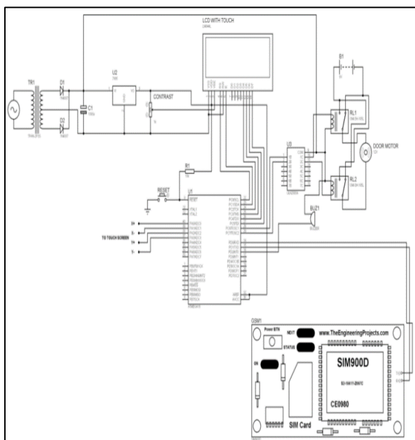
Fig 2: Circuit Diagram
